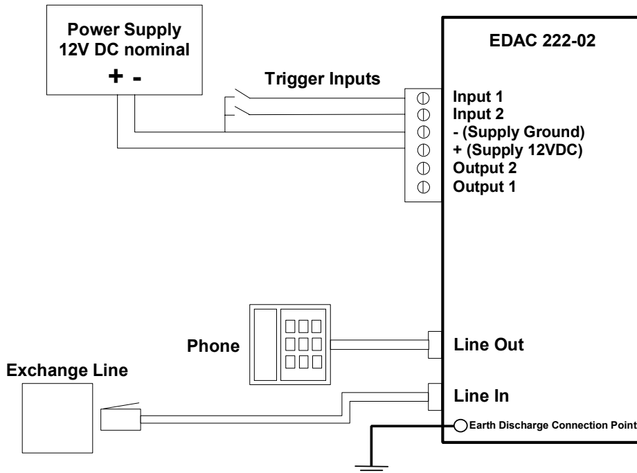
Figure 1: Typical EDAC 222-02 Installation
