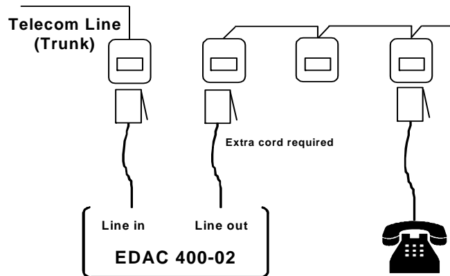
Figure 3: Secure Installation
