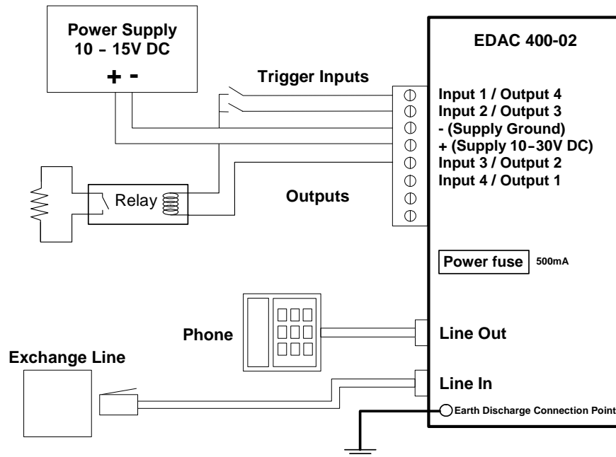
Figure 1: Typical EDAC 400-02 Installation
